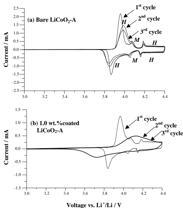
Fig. 10. Cyclic voltammograms of (a) bare \text{LiCoO}_2\text{-A} (b) 1.0 wt % boehmite-coated \text{LiCoO}_2\text{-A} .
