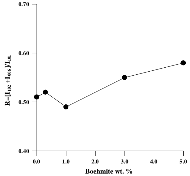
Fig. 3. Variation of the R -factor as a function of the coating level. Core material: \text{LiCoO}_2\text{-A} .
